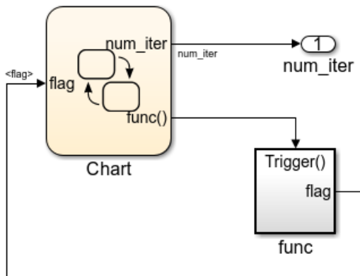
Model ex_while_loop_SF
